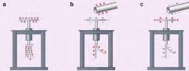
▲ Figure 9.10 a If there are no electrically charged objects held close to the plate the positive and negative charges are evenly spread throughout the electroscope and the gold leaf is not deflected. b If a positively charged object is brought close it attracts negative charges upwards onto the metal plate. This leaves both the metal rod and the gold leaf positively charged. They repel each other, so the leaf rises. c If a negatively charged object is brought close it repels the negatively charged electrons on the plate pushing them down onto the gold leaf and the bottom of the rod. These like charges repel and the leaf again moves upwards.
