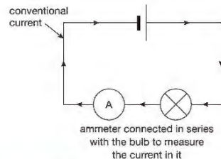
▲ Figure 7.3 An ammeter is used to measure current in a circuit. It has a very low resistance and so has almost no effect on the current.
